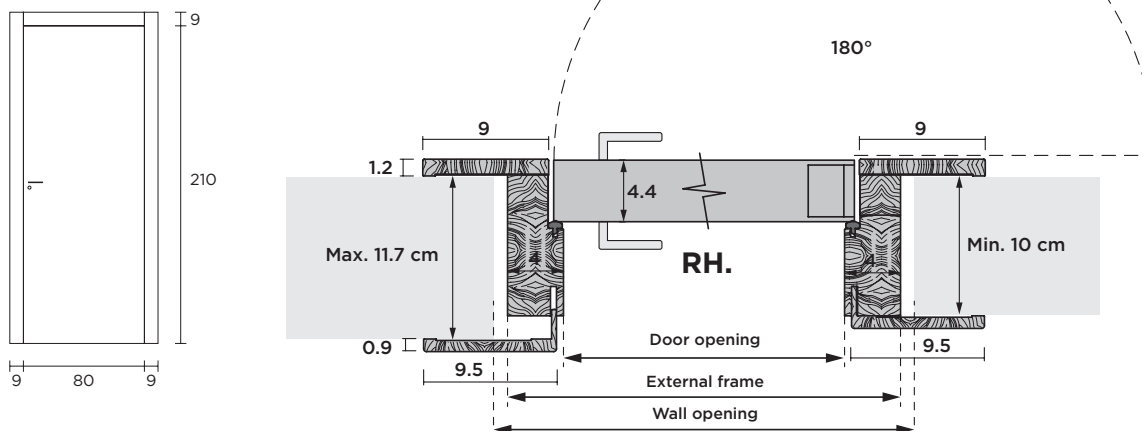
Concealed invisible hinges in satin chrome finish, 3D adjustable
